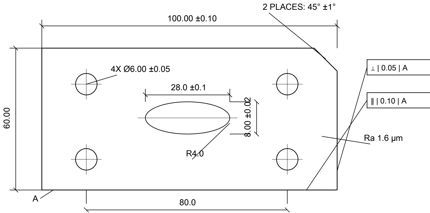
TOP VIEW
